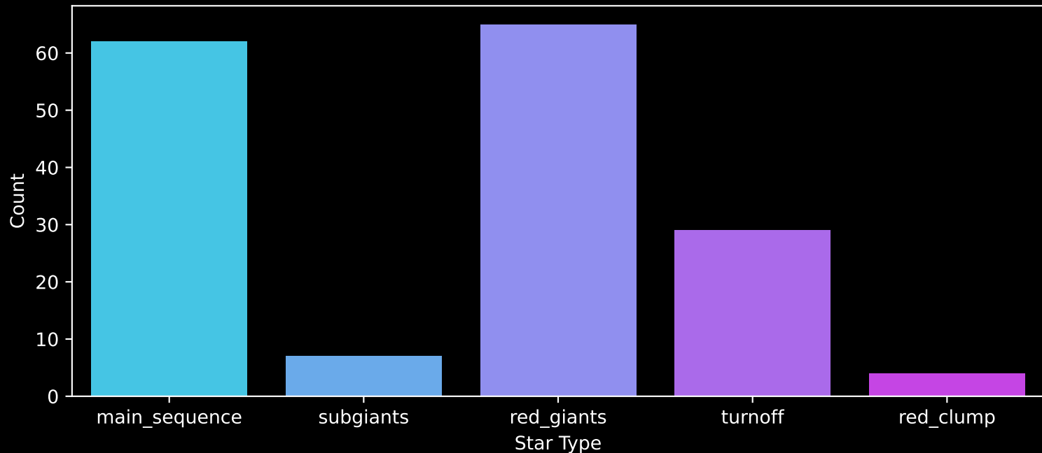
APOGEE DR17 Field: [281-24-O_TESS] Count plot of Star Type
