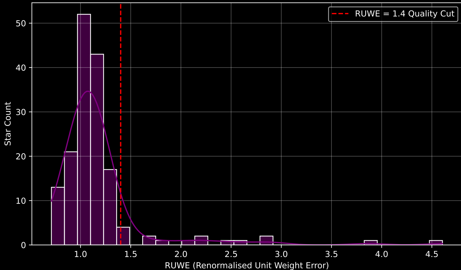
GAPOGEE DR17 Field [281-24-O_TESS] RUWE Distribution (n= 162)
