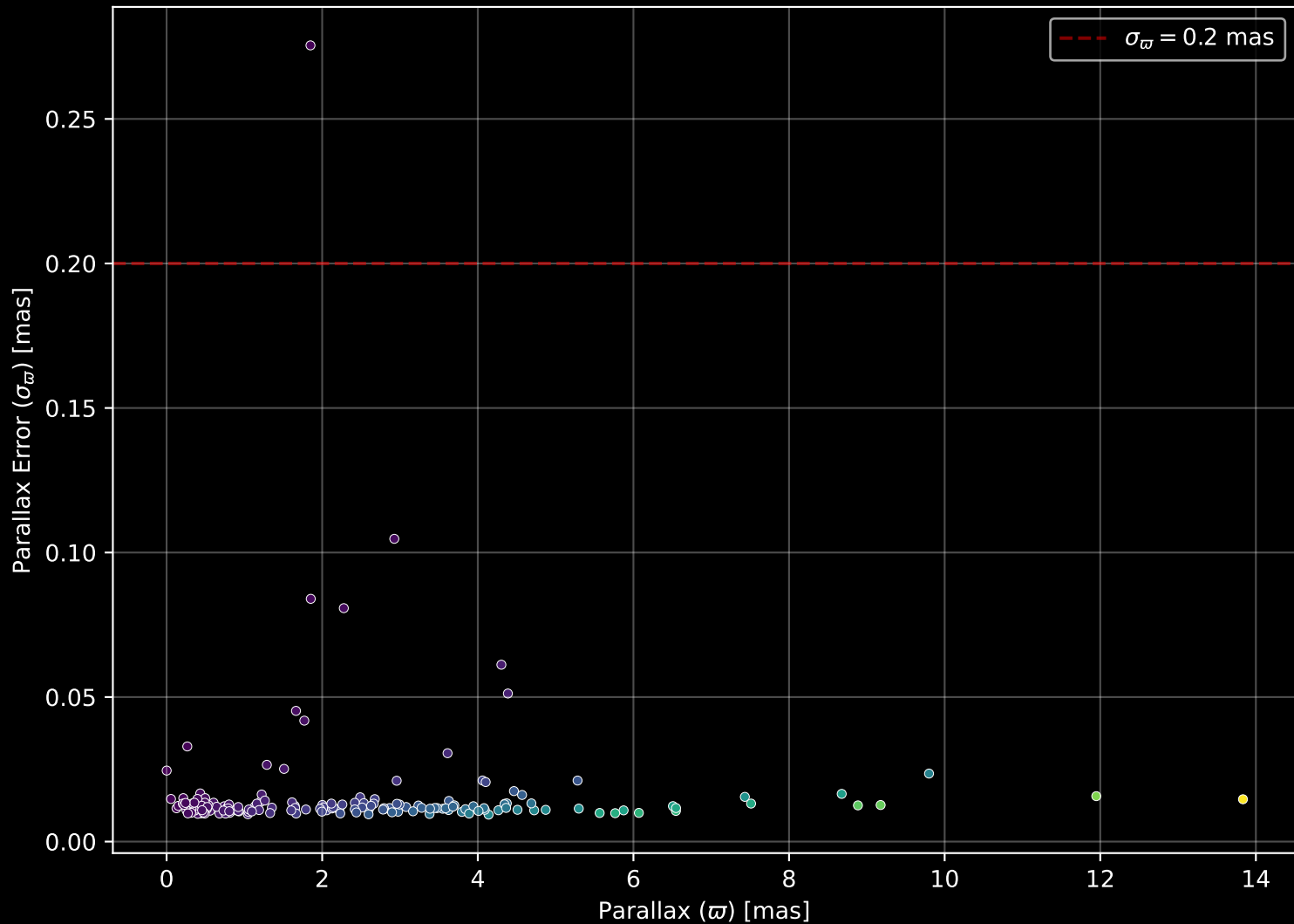
APOGEE DR17 Field: [281-24-O_TESS] Parallax Quality (n= 167)
