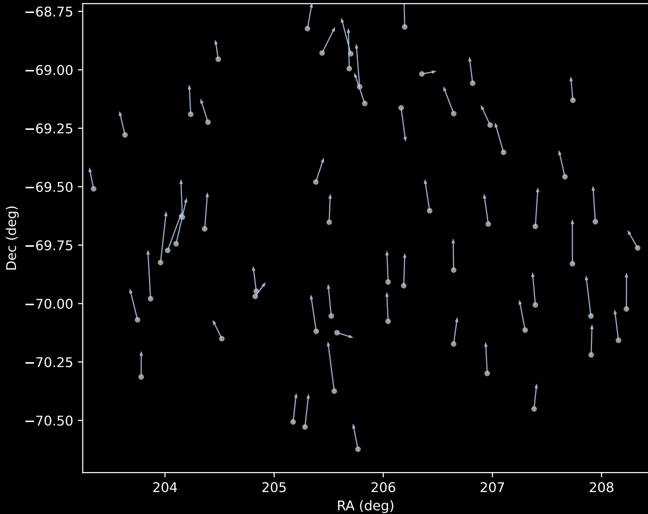
APOGEE DR17 Cluster 1 Proper Motion Vectors (n=59)
